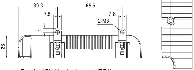
Terminal Pin No. Assignment(TB1)
